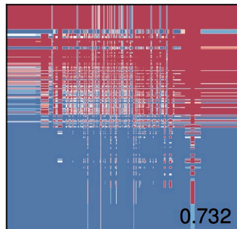
Binarized features
