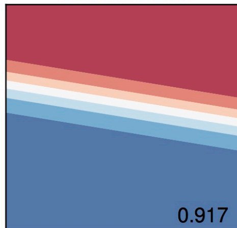
Raw features
