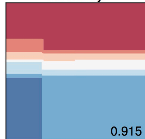
Binarsity
